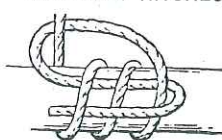
HALYARD BEND
