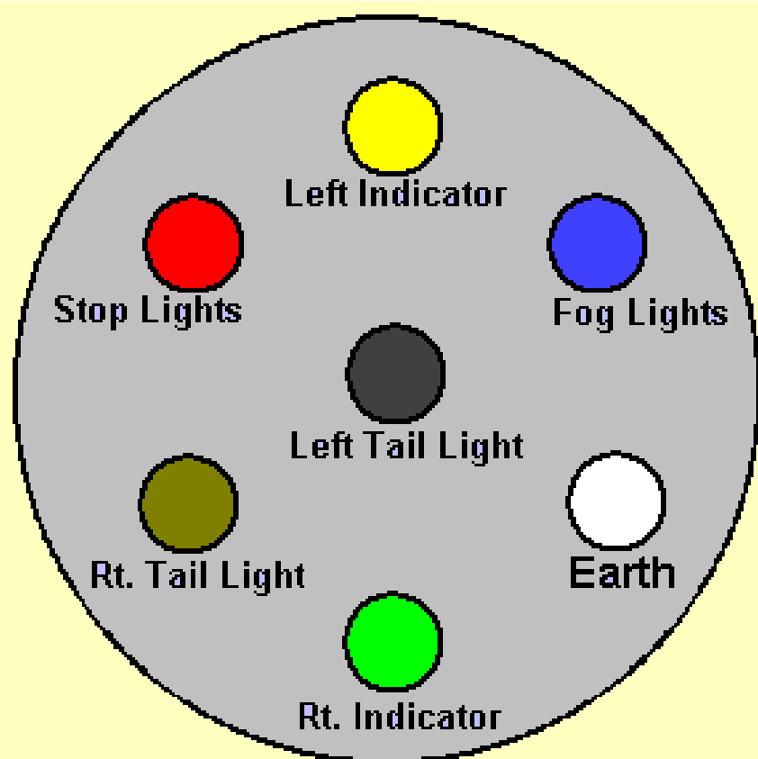
Trailer Socket (FACING) and Trailer Plug (Rear of)
